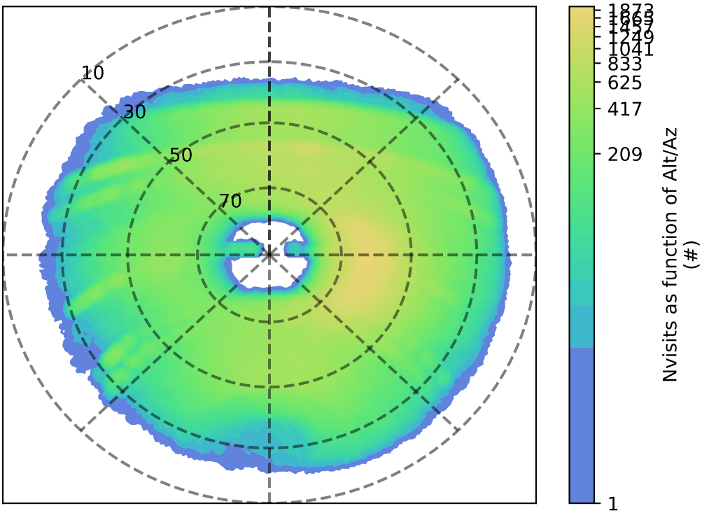
roll_uniform_eh_acc0.0_mjdp0_v3.4_10yrs y: Nvisits as function of Alt/Az
