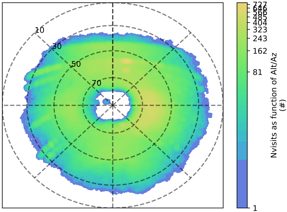
roll_uniform_eh_acc0.0_mjdp0_v3.4_10yrs u: Nvisits as function of Alt/Az
