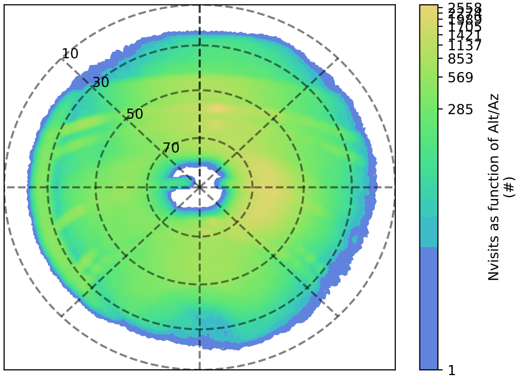
roll_uniform_eh_acc0.0_mjdp0_v3.4_10yrs r: Nvisits as function of Alt/Az
