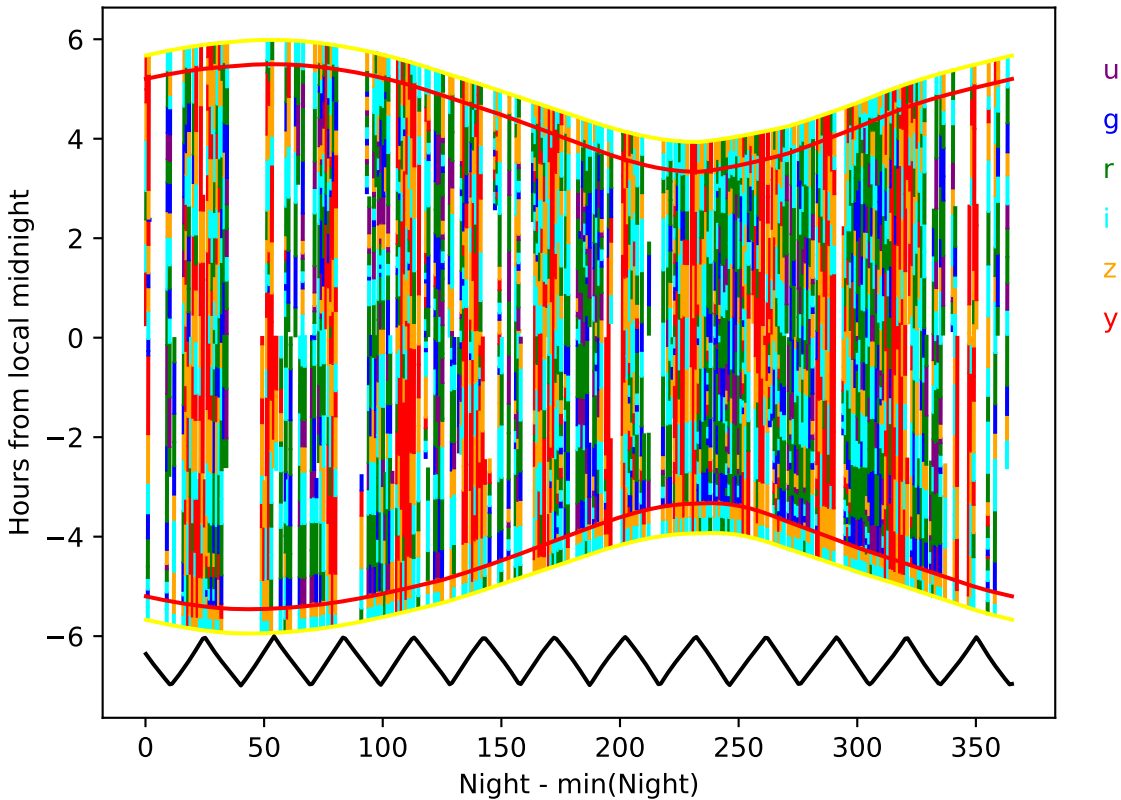
roll_uniform_eh_acc0.0_mjdp0_v3.4_10yrs year 4-5: Hourglass
