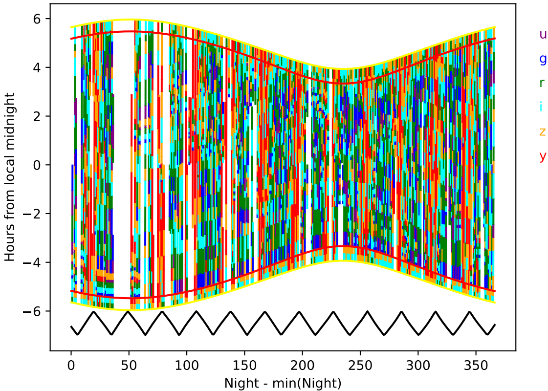
roll_uniform_eh_acc0.0_mjdp0_v3.4_10yrs year 2-3: Hourglass
