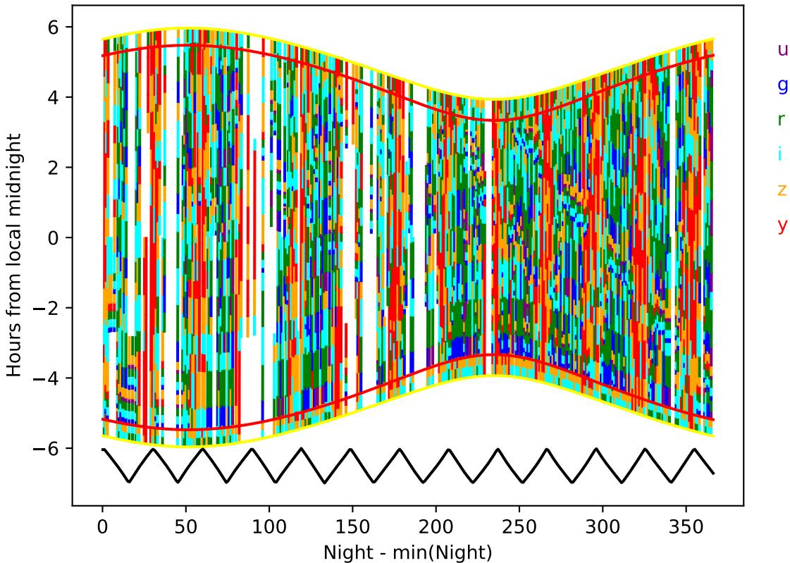
roll_uniform_eh_acc0.0_mjdp0_v3.4_10yrs year 1-2: Hourglass
