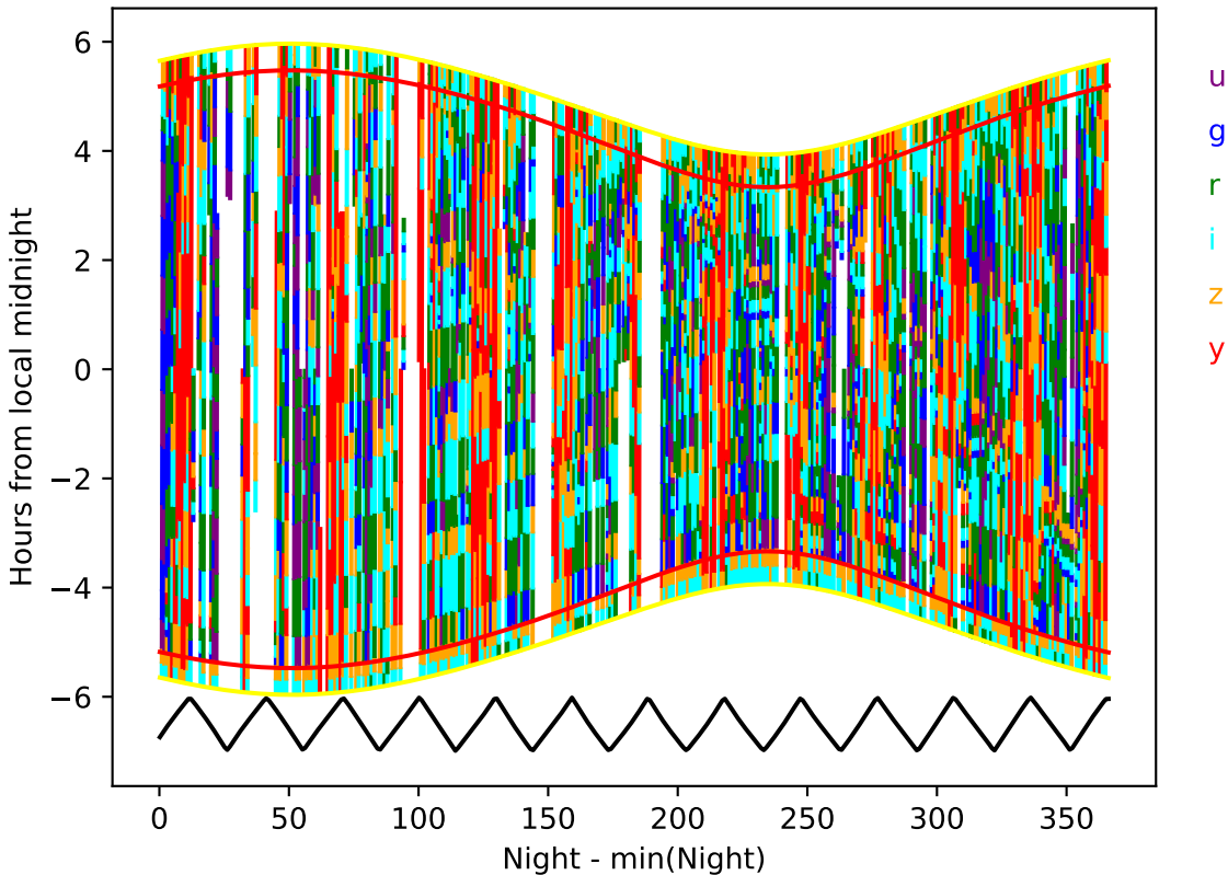
roll_uniform_eh_acc0.0_mjdp0_v3.4_10yrs year 0-1: Hourglass
