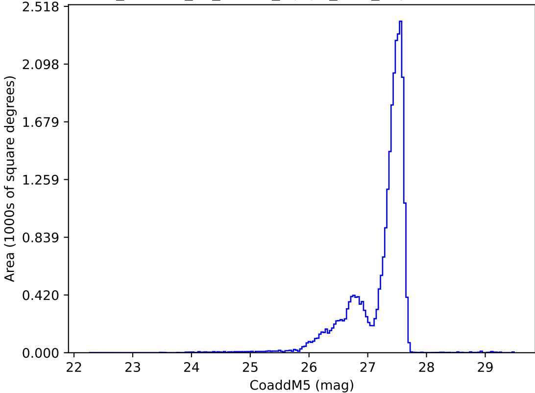
roll_uniform_eh_acc0.0_mjdp0_v3.4_10yrs : CoaddM5
