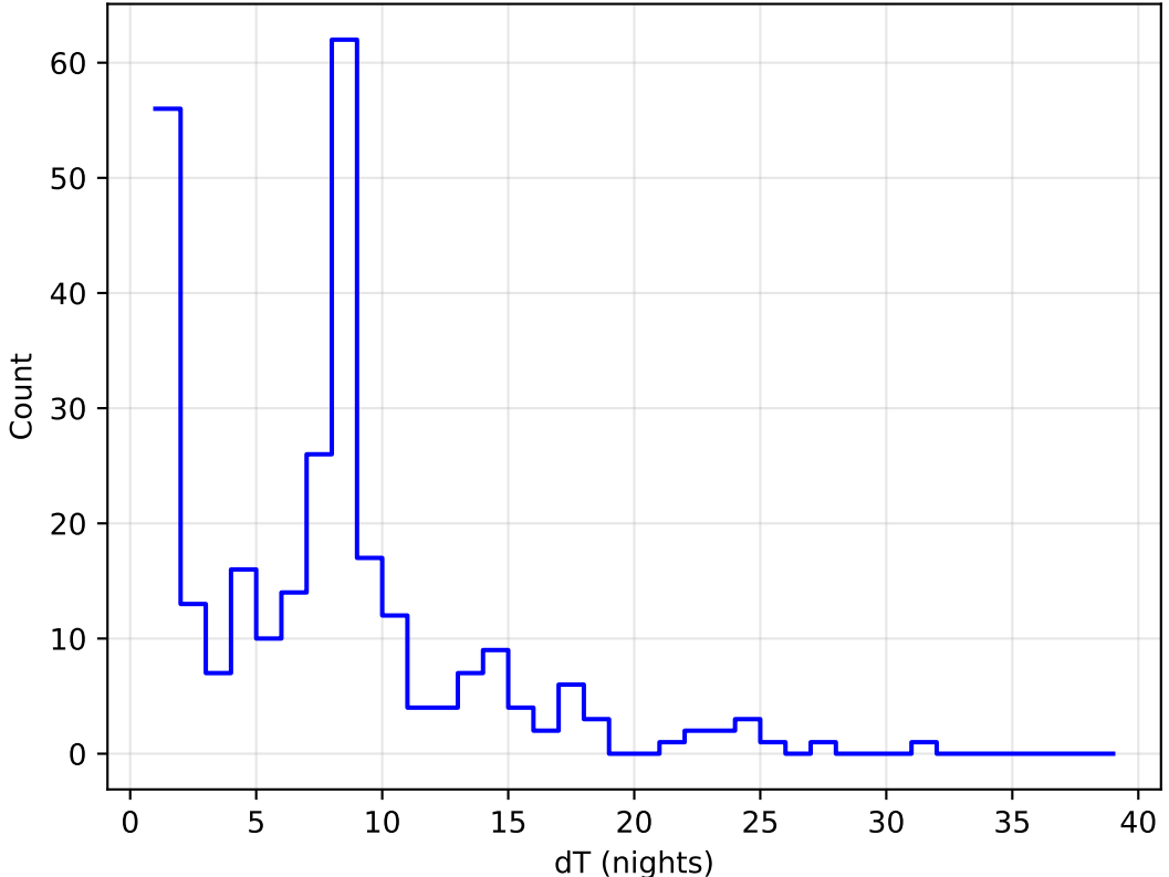
roll_uniform_eh_acc0.0_mjdp0_v3.4_10yrs all bands: DD:XMM_LSS Delta Nights Histogram
