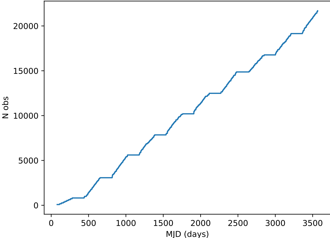
roll_uniform_eh_acc0.0_mjdp0_v3.4_10yrs all bands: DD:XMM_LSS Cumulative NVisits
