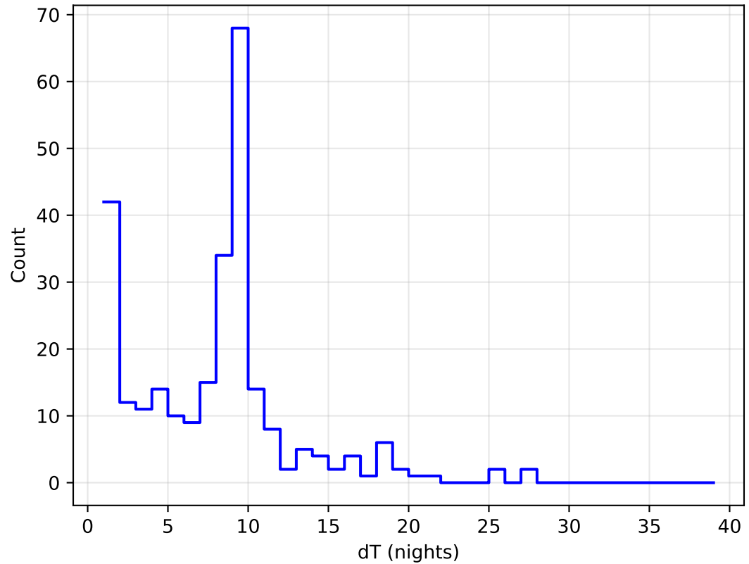
roll_uniform_eh_acc0.0_mjdp0_v3.4_10yrs all bands: DD:ELAISS1 Delta Nights Histogram
