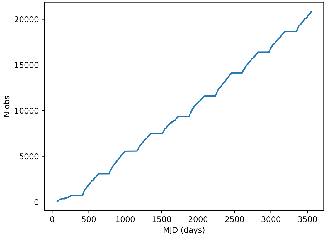
roll_uniform_eh_acc0.0_mjdp0_v3.4_10yrs all bands: DD:ELAISS1 Cumulative NVisits
