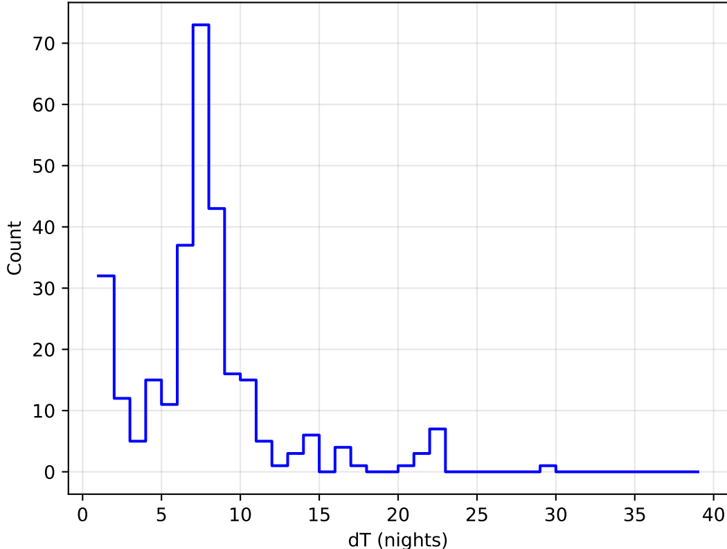
roll_uniform_eh_acc0.0_mjdp0_v3.4_10yrs all bands: DD:EDFS Delta Nights Histogram
