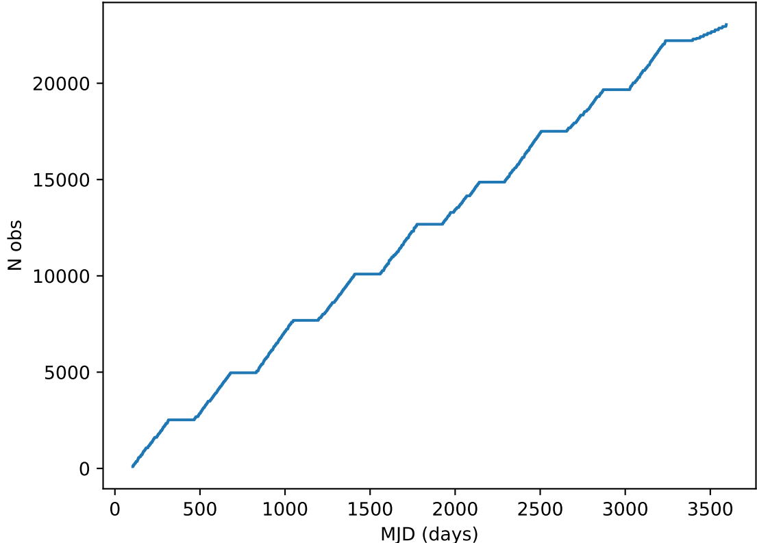
roll_uniform_eh_acc0.0_mjdp0_v3.4_10yrs all bands: DD:EDFS Cumulative NVisits
