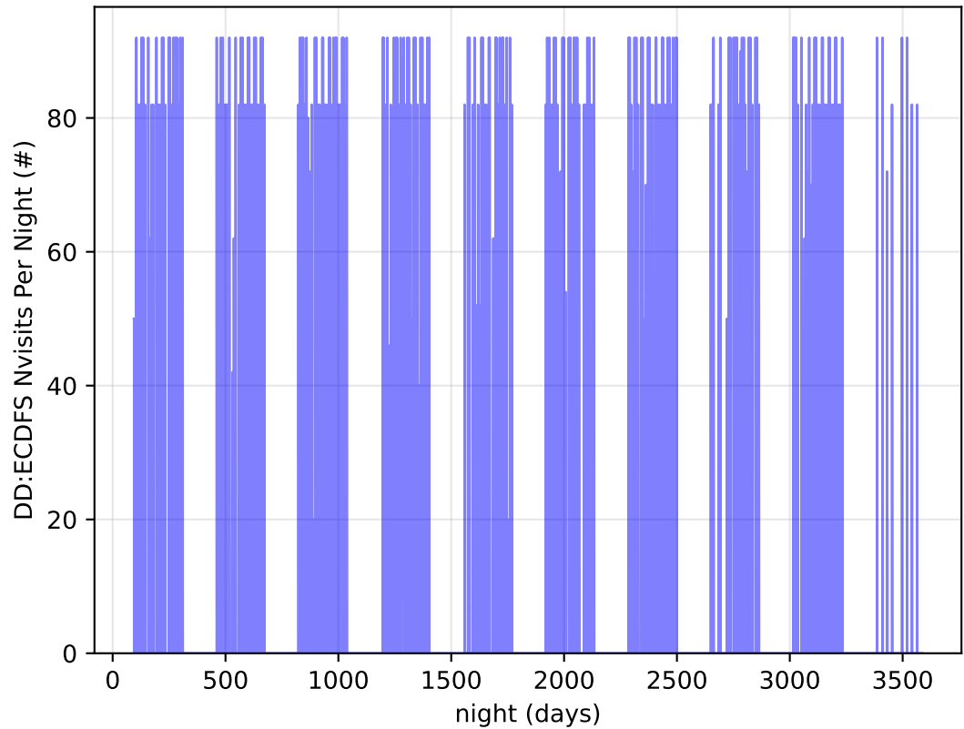
roll_uniform_eh_acc0.0_mjdp0_v3.4_10yrs all bands: DD:ECDFS Nvisits Per Night
