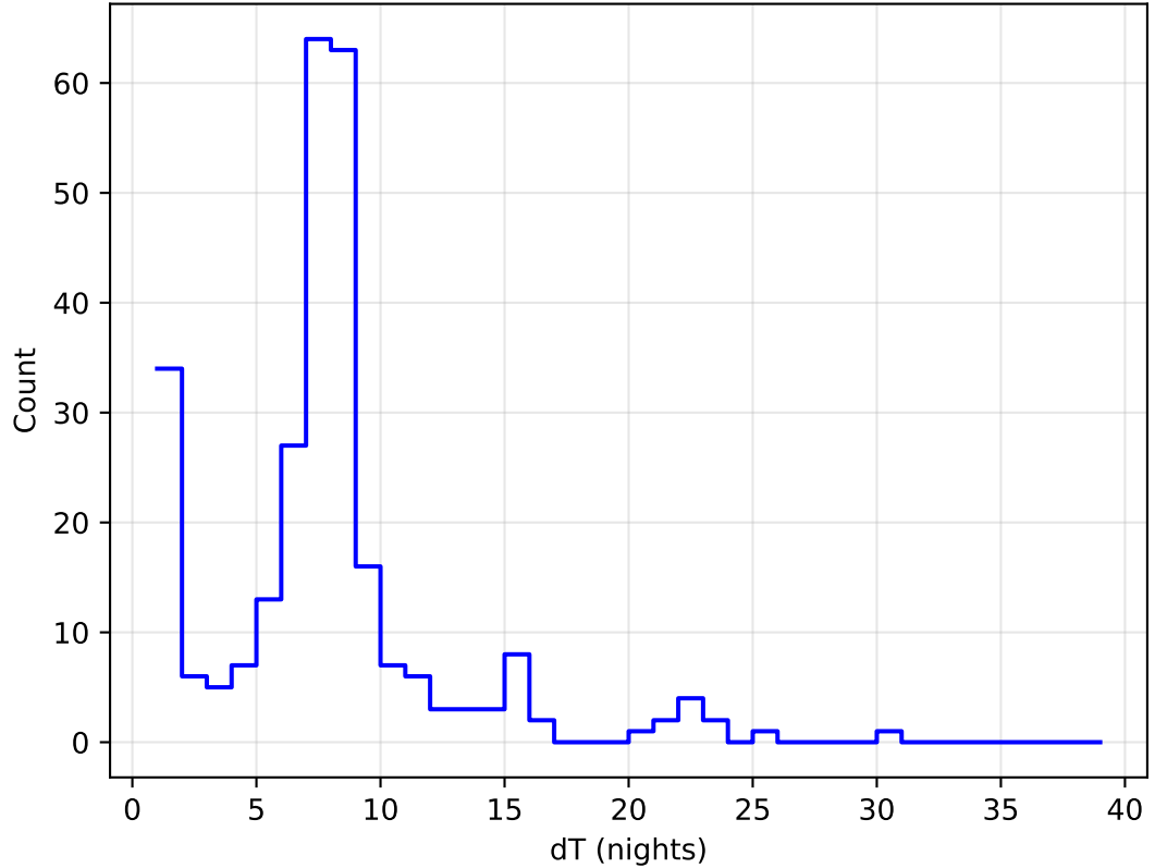
roll_uniform_eh_acc0.0_mjdp0_v3.4_10yrs all bands: DD:ECDFS Delta Nights Histogram
