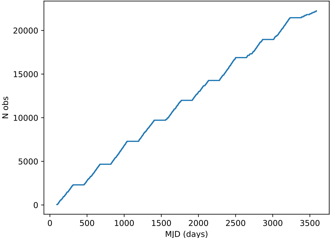
roll_uniform_eh_acc0.0_mjdp0_v3.4_10yrs all bands: DD:ECDFS Cumulative NVisits
