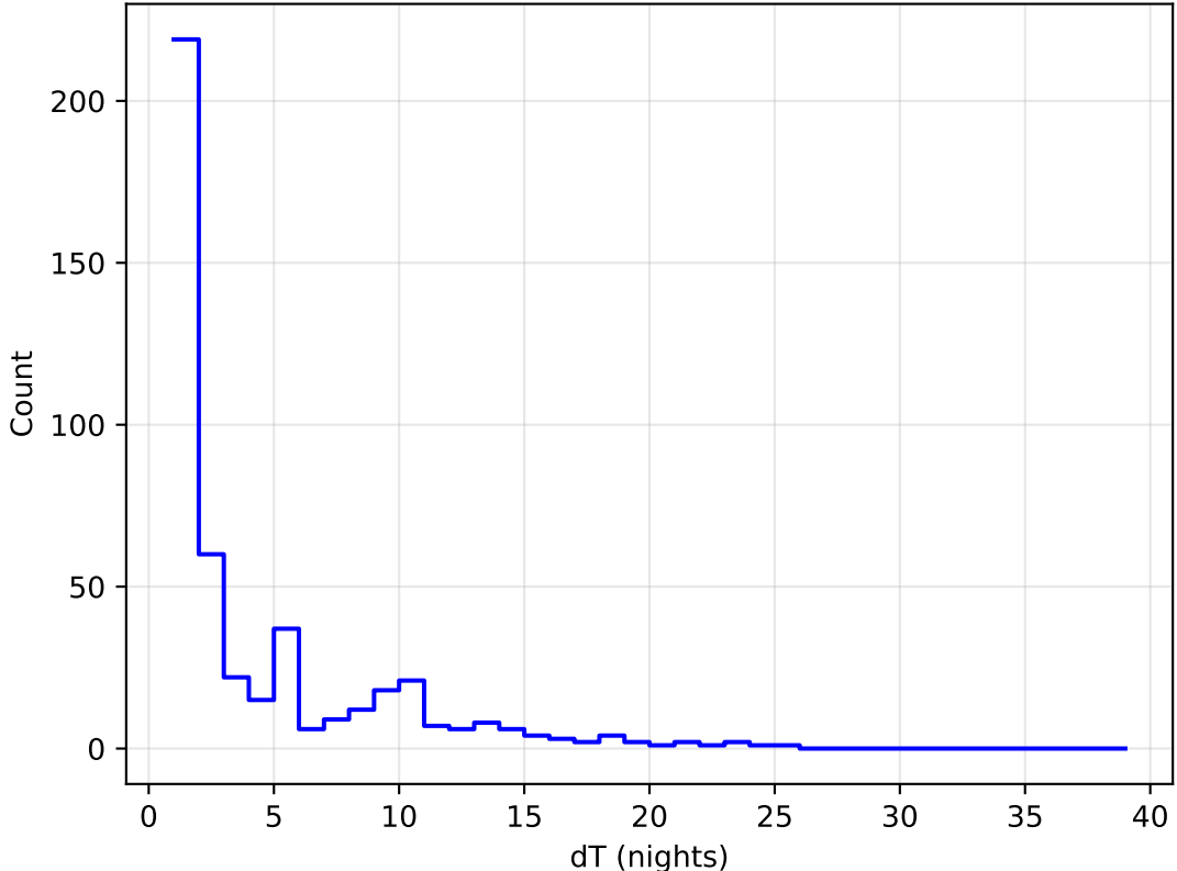
roll_uniform_eh_acc0.0_mjdp0_v3.4_10yrs all bands: DD: COSMOS Delta Nights Histogram
