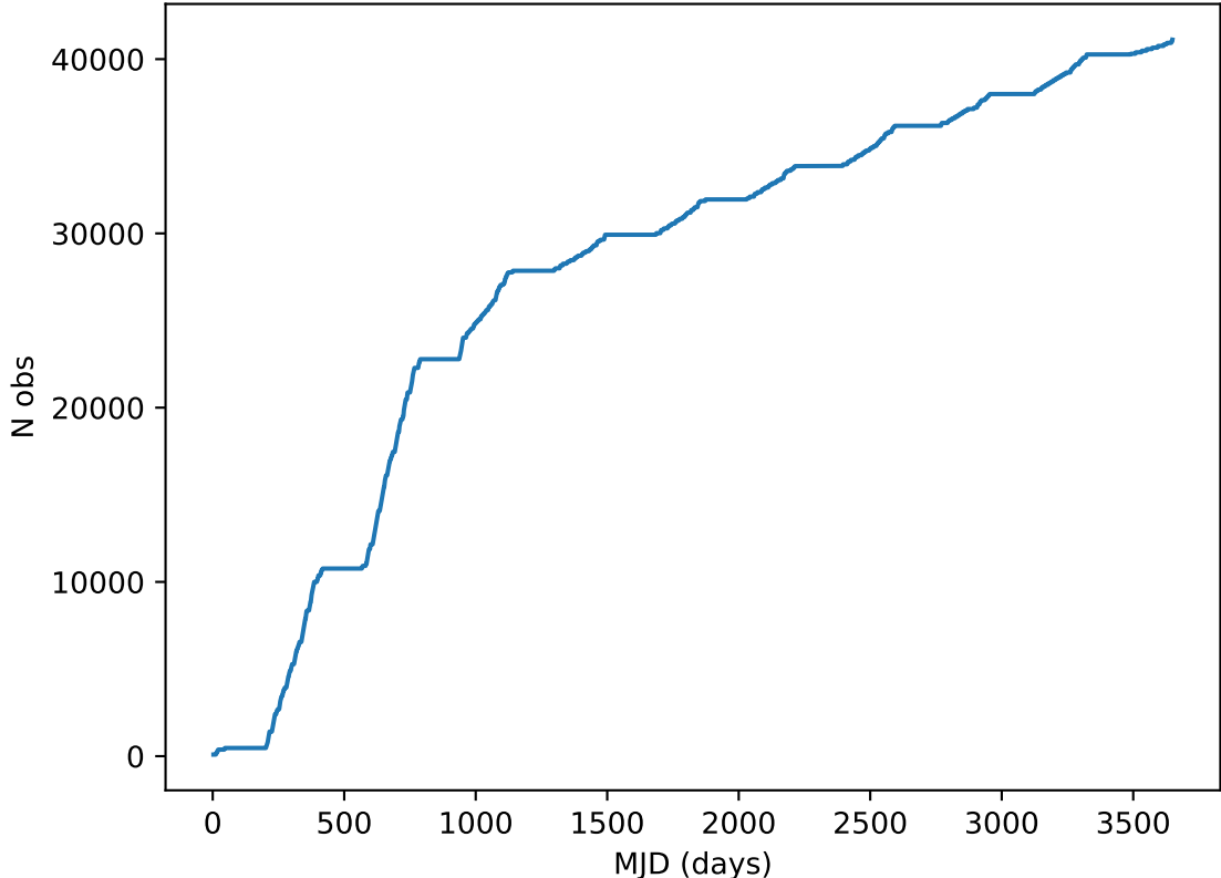
roll_uniform_eh_acc0.0_mjdp0_v3.4_10yrs all bands: DD: COSMOS Cumulative NVisits
