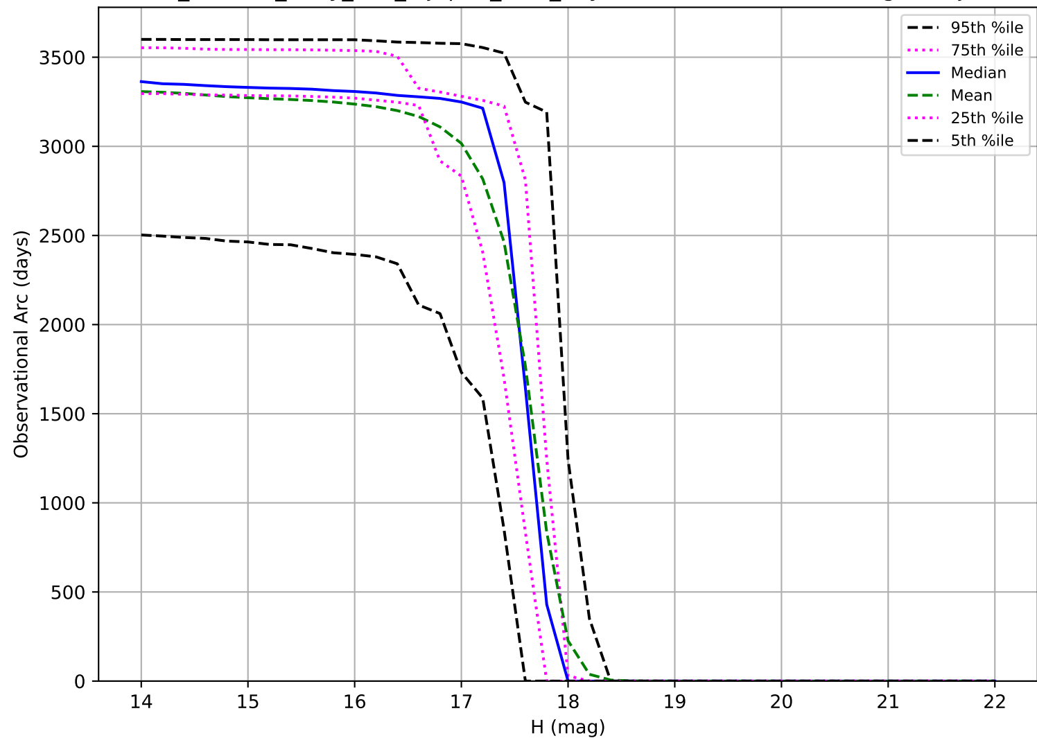
roll_uniform_early_half_mjdp67_v3.4_10yrs: Observational Arc Length Trojan
