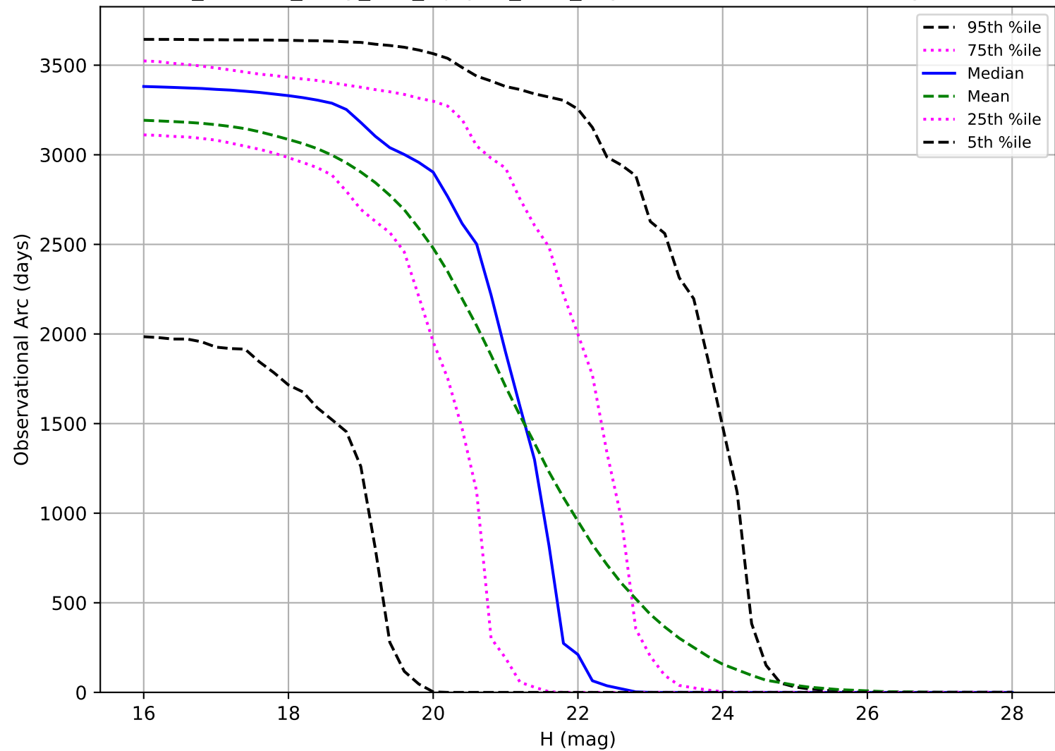
roll_uniform_early_half_mjdp67_v3.4_10yrs: Observational Arc Length PHA
