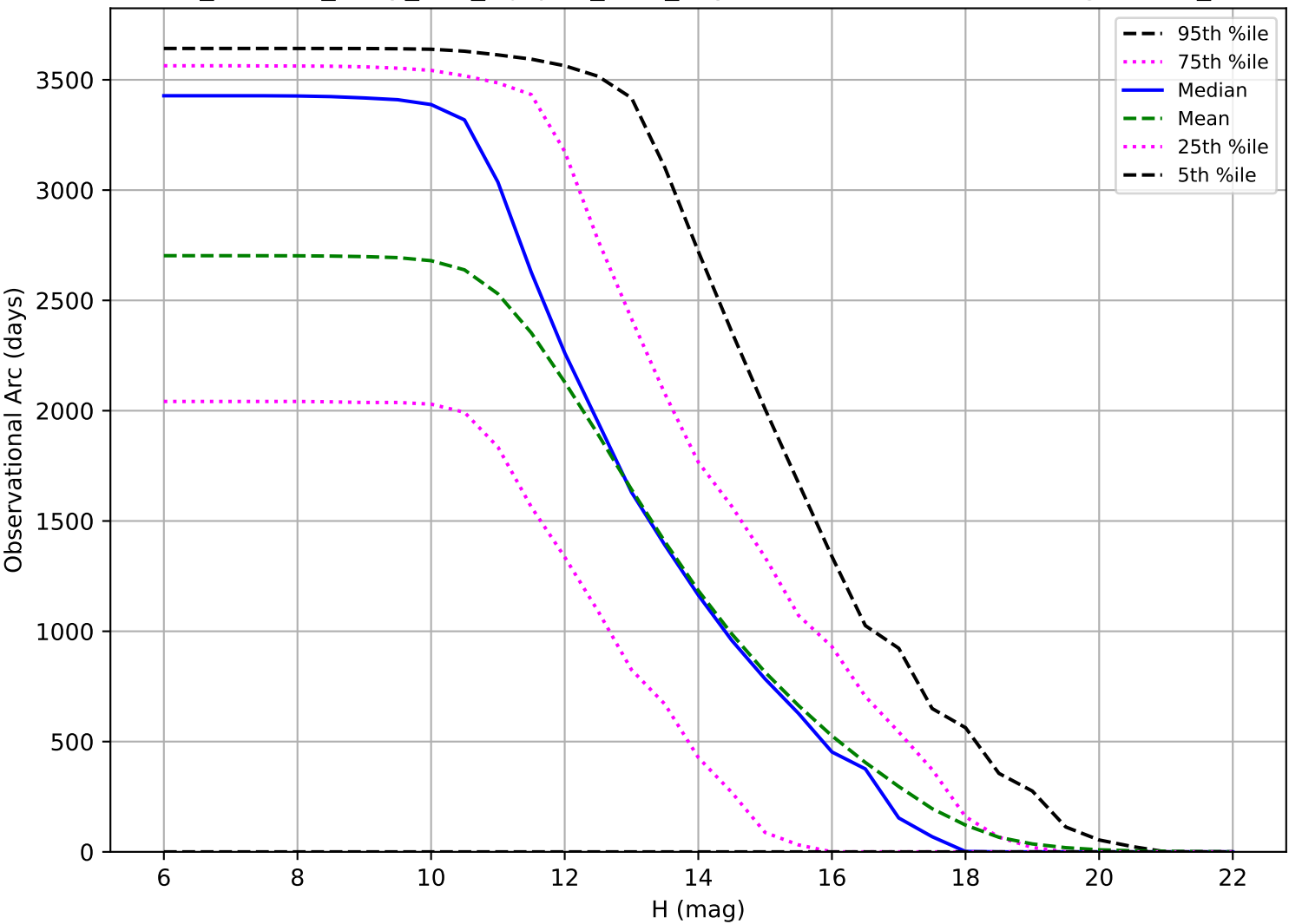
roll_uniform_early_half_mjdp67_v3.4_10yrs: Observational Arc Length OCC_r5
