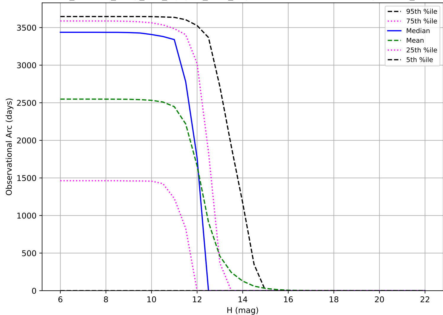
roll_uniform_early_half_mjdp67_v3.4_10yrs: Observational Arc Length OCC_r20
