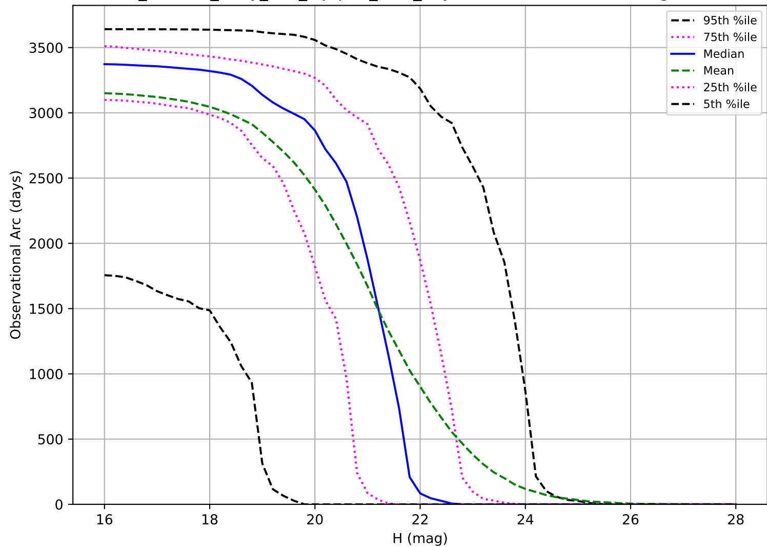
roll_uniform_early_half_mjdp67_v3.4_10yrs: Observational Arc Length NEO
