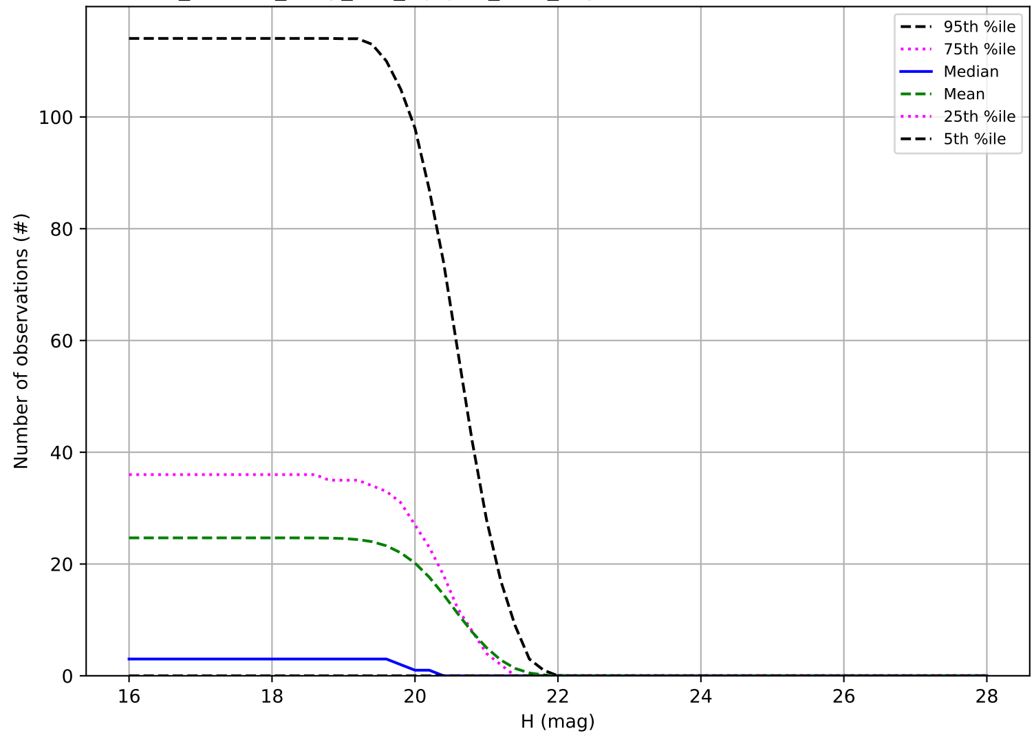
roll_uniform_early_half_mjdp67_v3.4_10yrs: Number of observations Vatira
