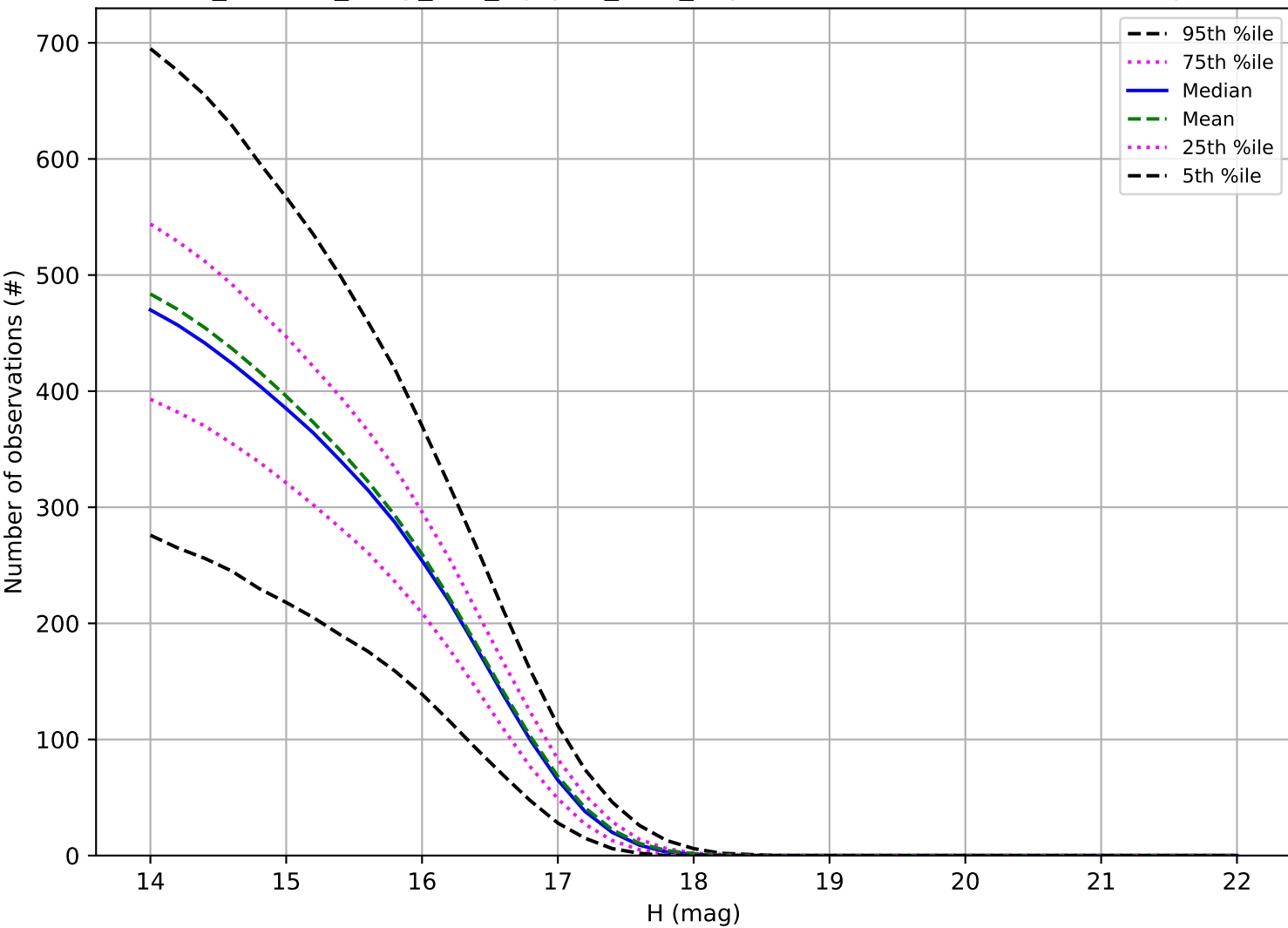
roll_uniform_early_half_mjdp67_v3.4_10yrs: Number of observations Trojan
