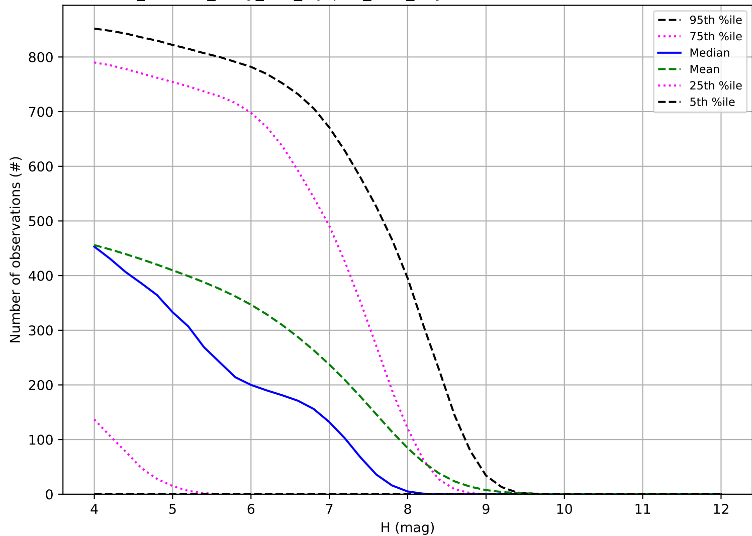
roll_uniform_early_half_mjdp67_v3.4_10yrs: Number of observations TNO
