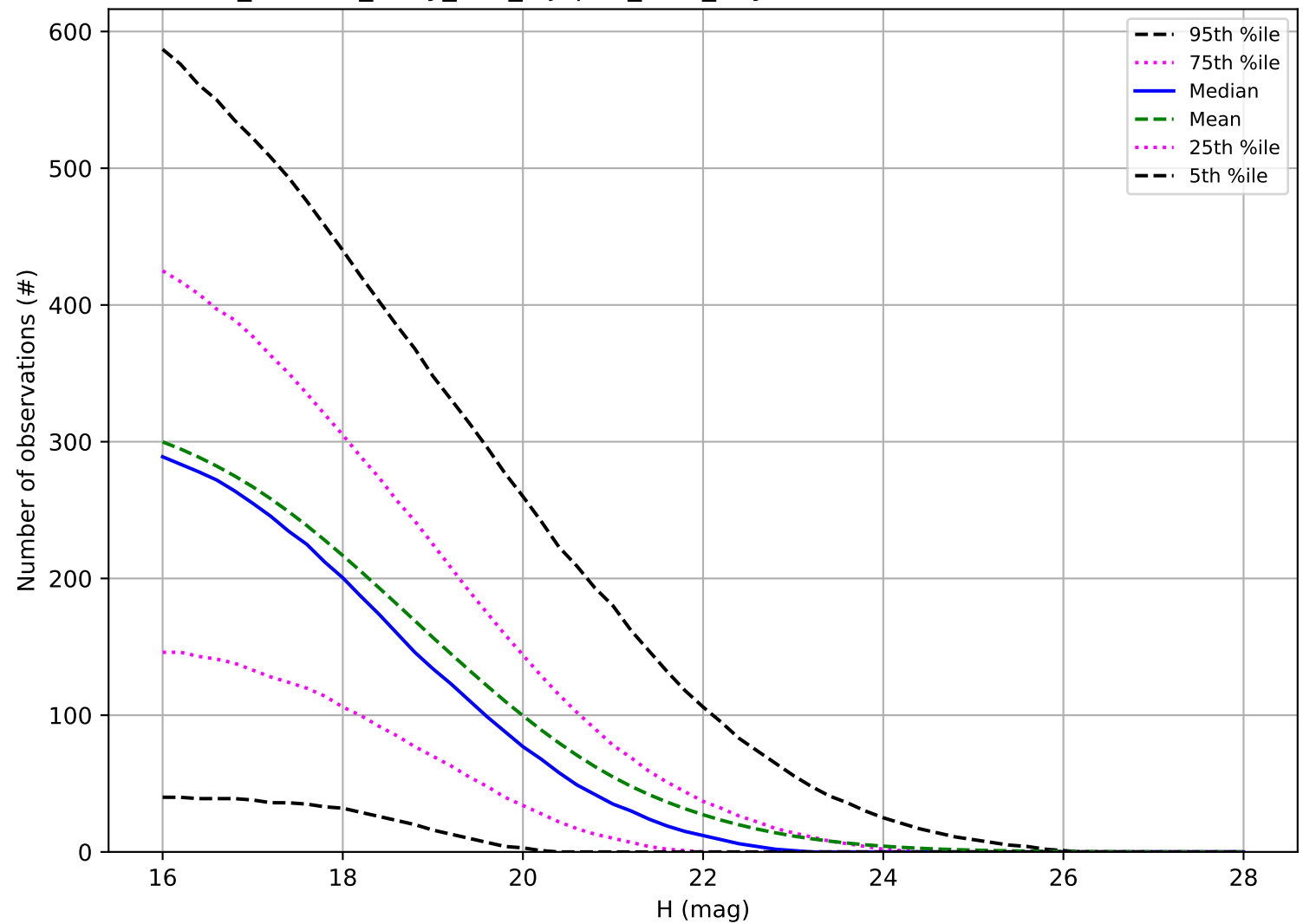
roll_uniform_early_half_mjdp67_v3.4_10yrs: Number of observations PHA
