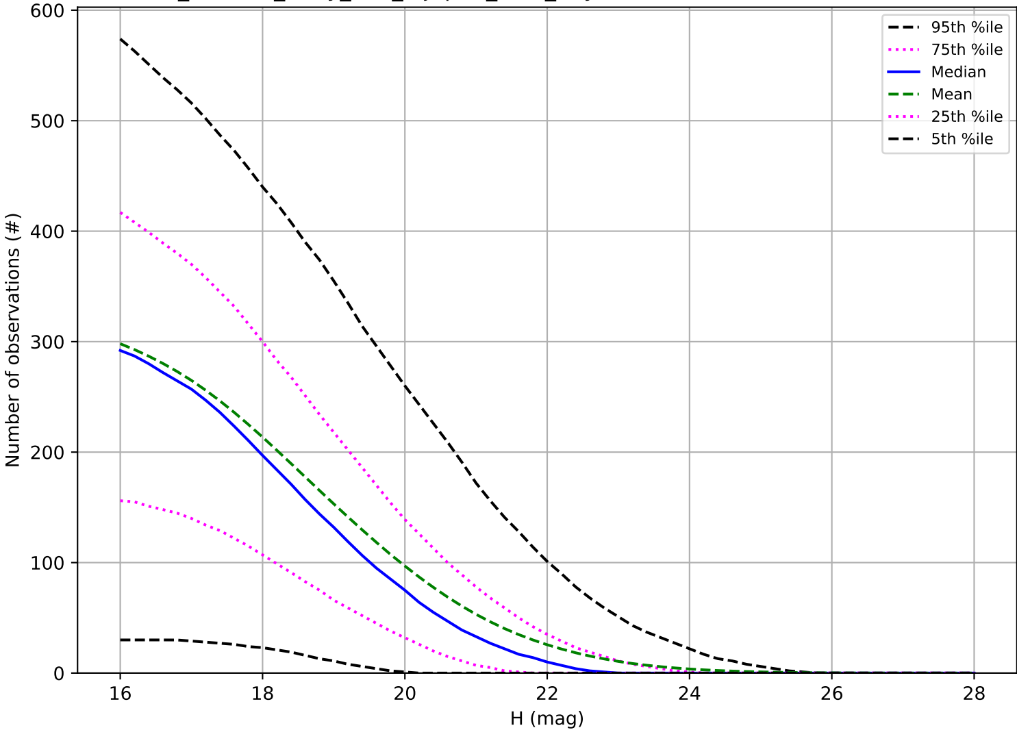
roll_uniform_early_half_mjdp67_v3.4_10yrs: Number of observations NEO
