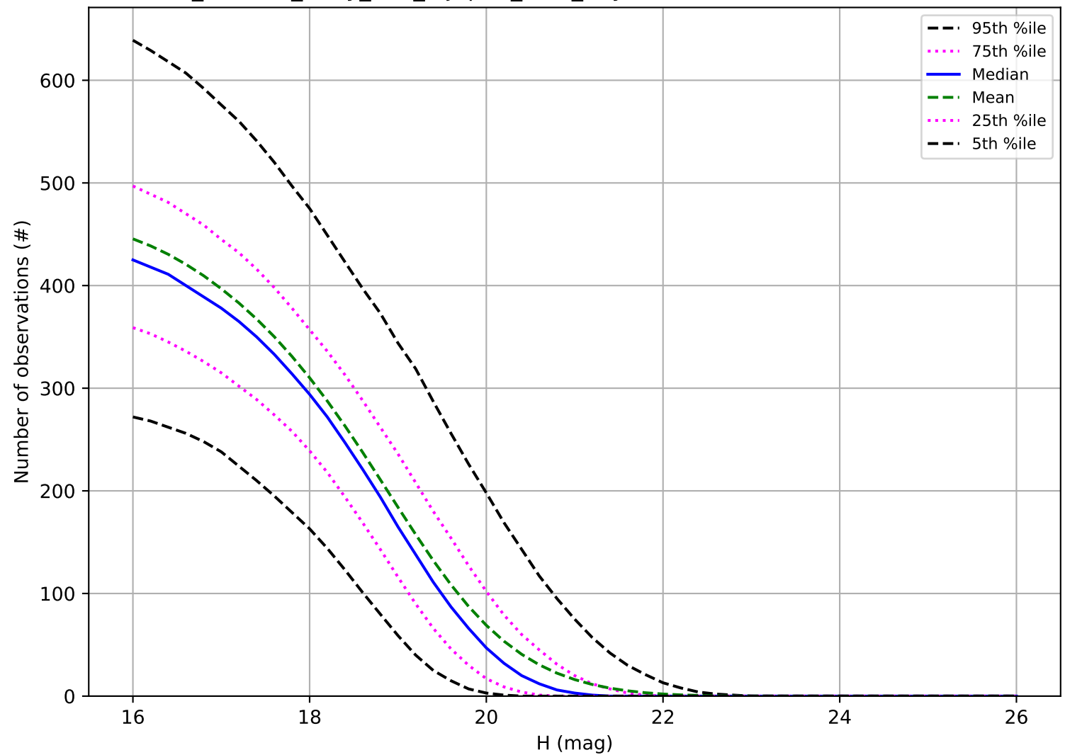
roll_uniform_early_half_mjdp67_v3.4_10yrs: Number of observations MBA
