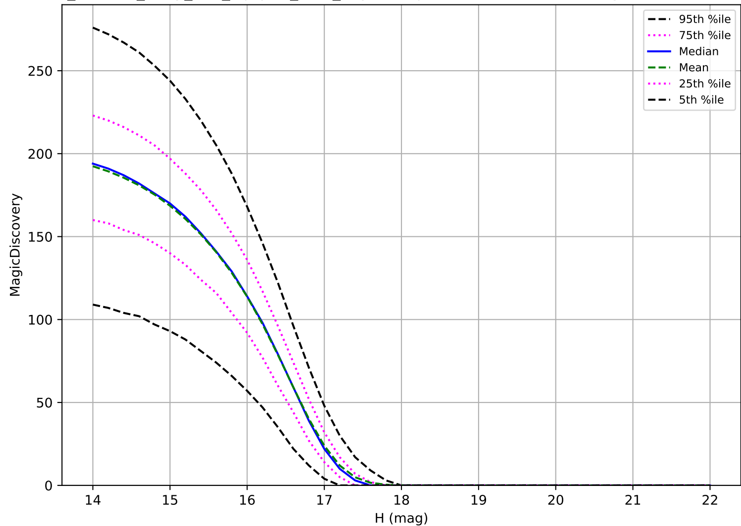
roll_uniform_early_half_mjdp67_v3.4_10yrs: Trojan 6 detections in 60 nights detection loss
