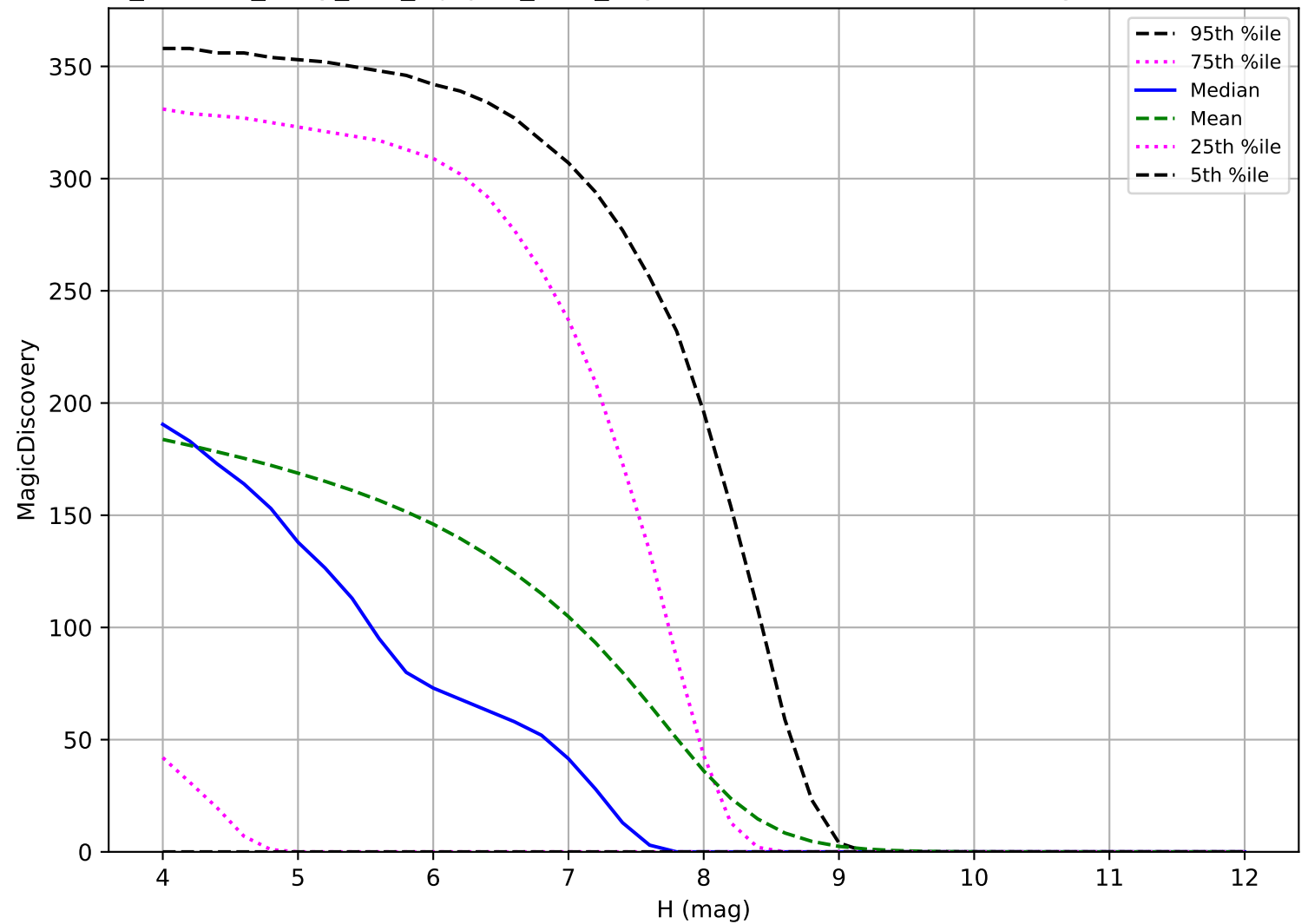
roll_uniform_early_half_mjdp67_v3.4_10yrs: TNO 6 detections in 60 nights detection loss
