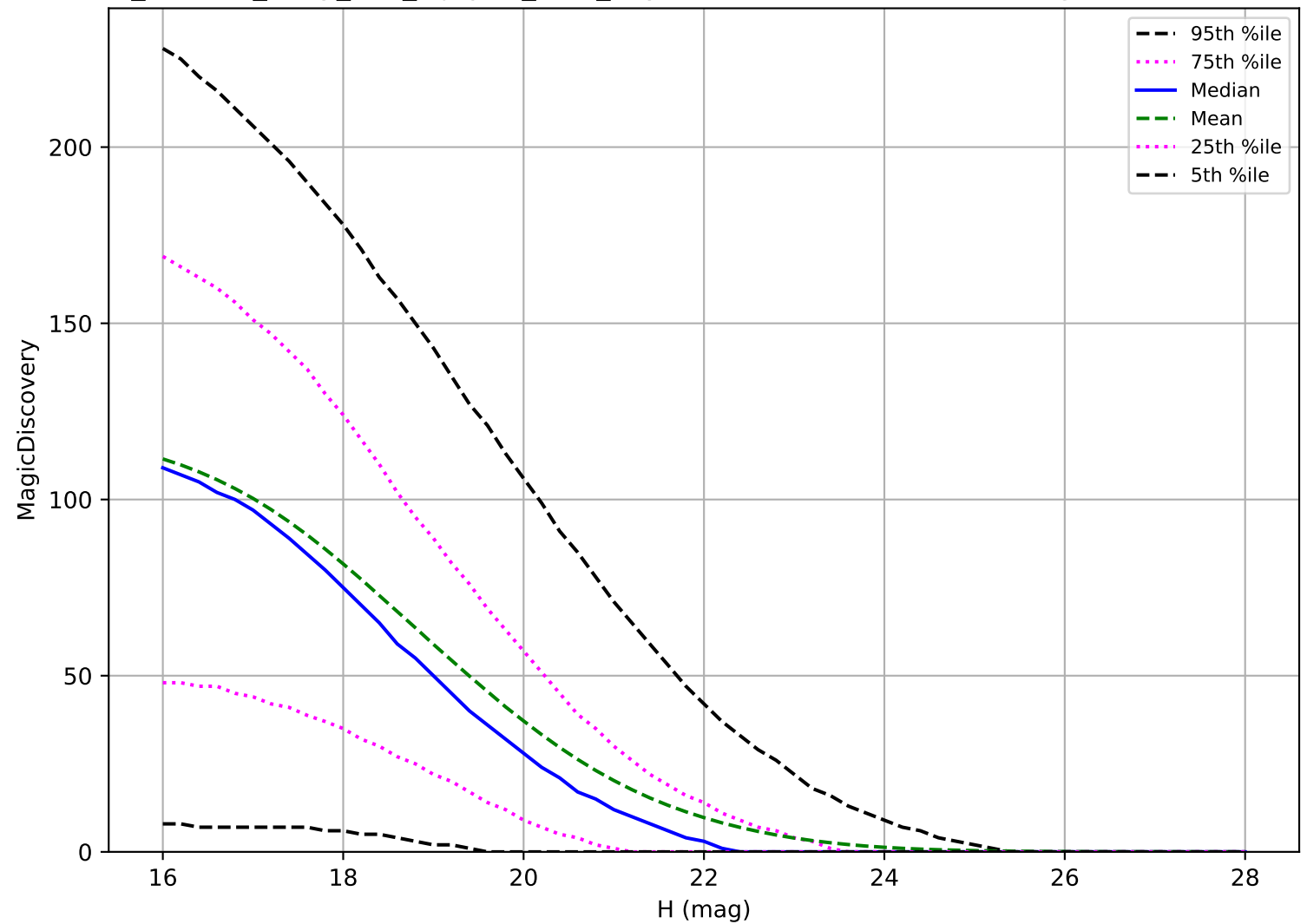
roll_uniform_early_half_mjdp67_v3.4_10yrs: PHA 6 detections in 60 nights detection loss
