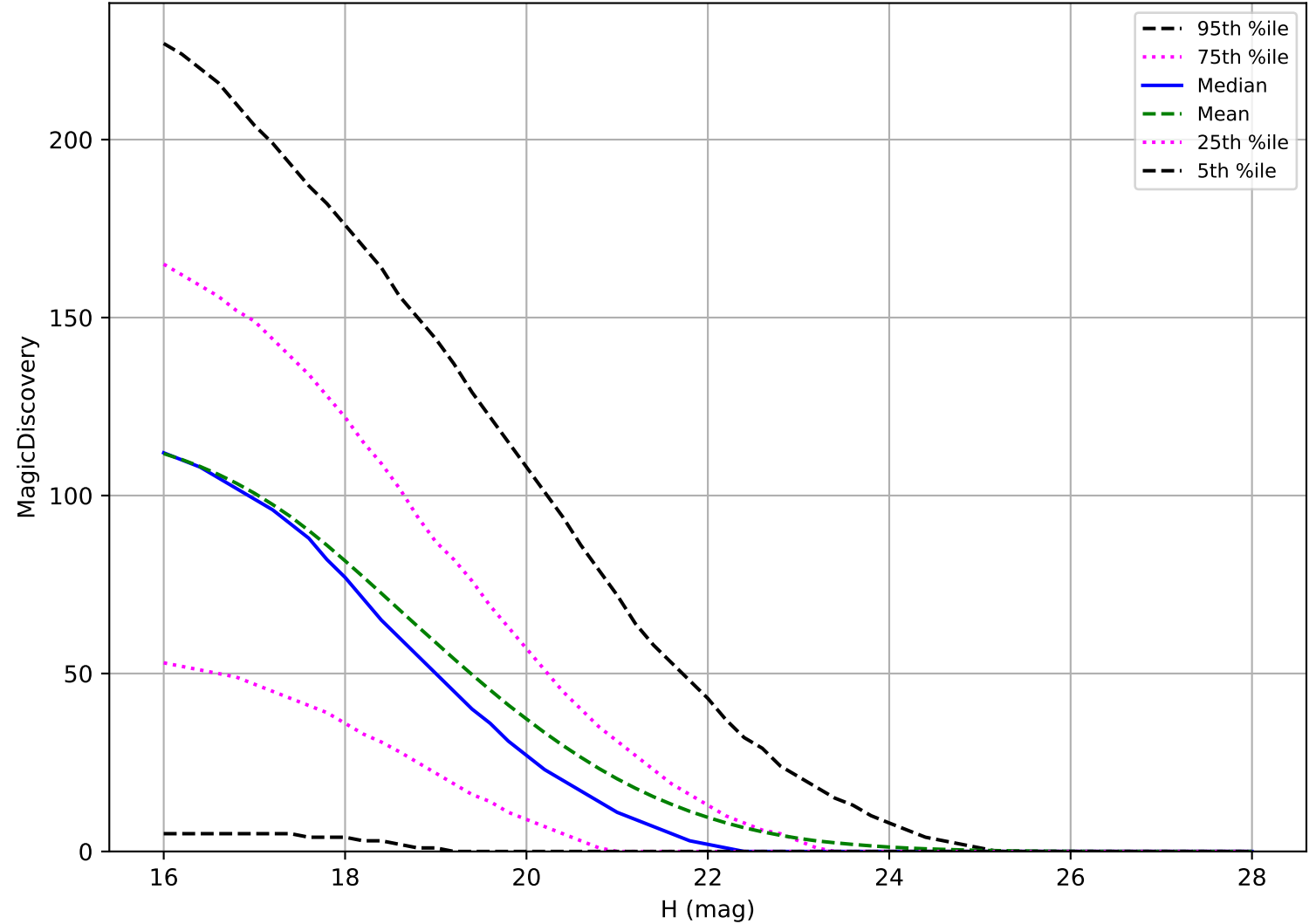
roll_uniform_early_half_mjdp67_v3.4_10yrs: NEO 6 detections in 60 nights detection loss
