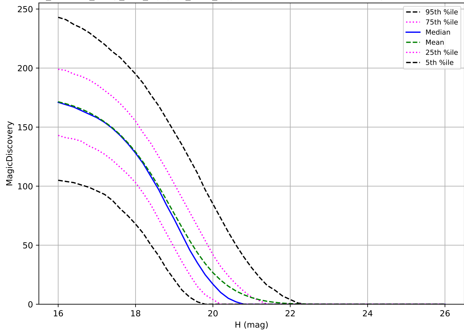
roll_uniform_early_half_mjdp67_v3.4_10yrs: MBA 6 detections in 60 nights detection loss
