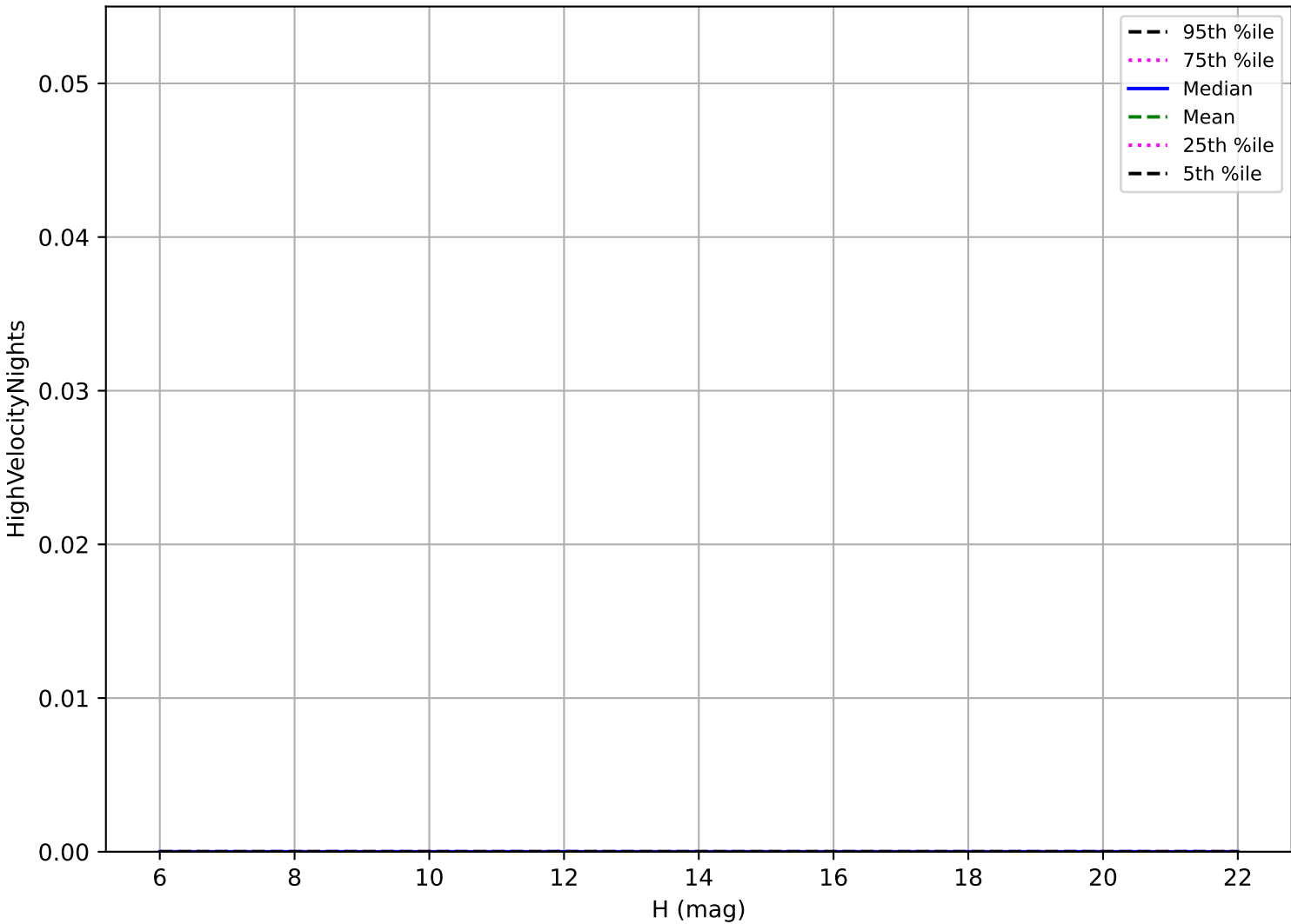
roll_uniform_early_half_mjdp67_v3.4_10yrs: OCC_r5 High velocity pair detection loss
