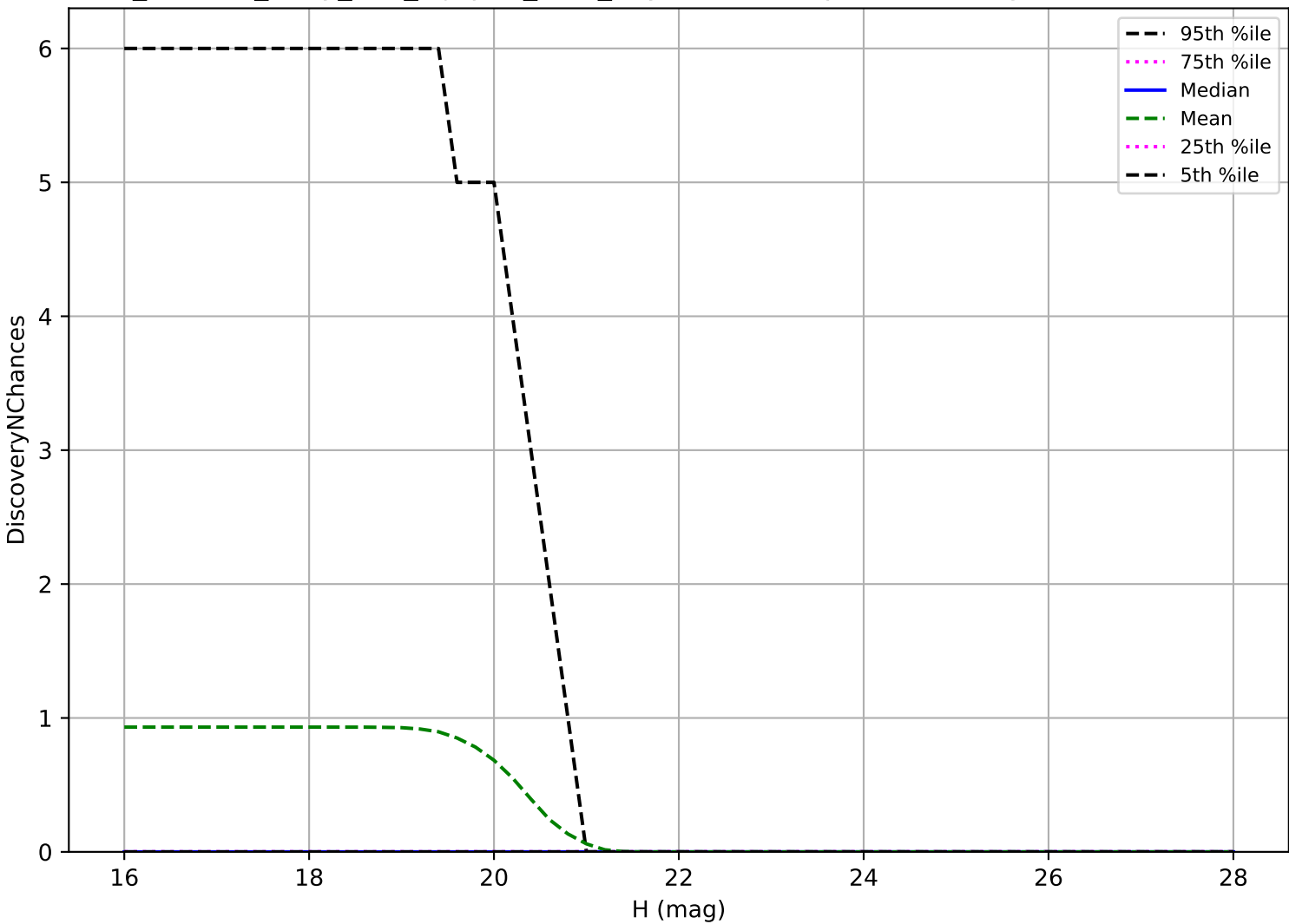
roll_uniform_early_half_mjdp67_v3.4_10yrs: Vatira 3 pairs in 15 nights detection loss
