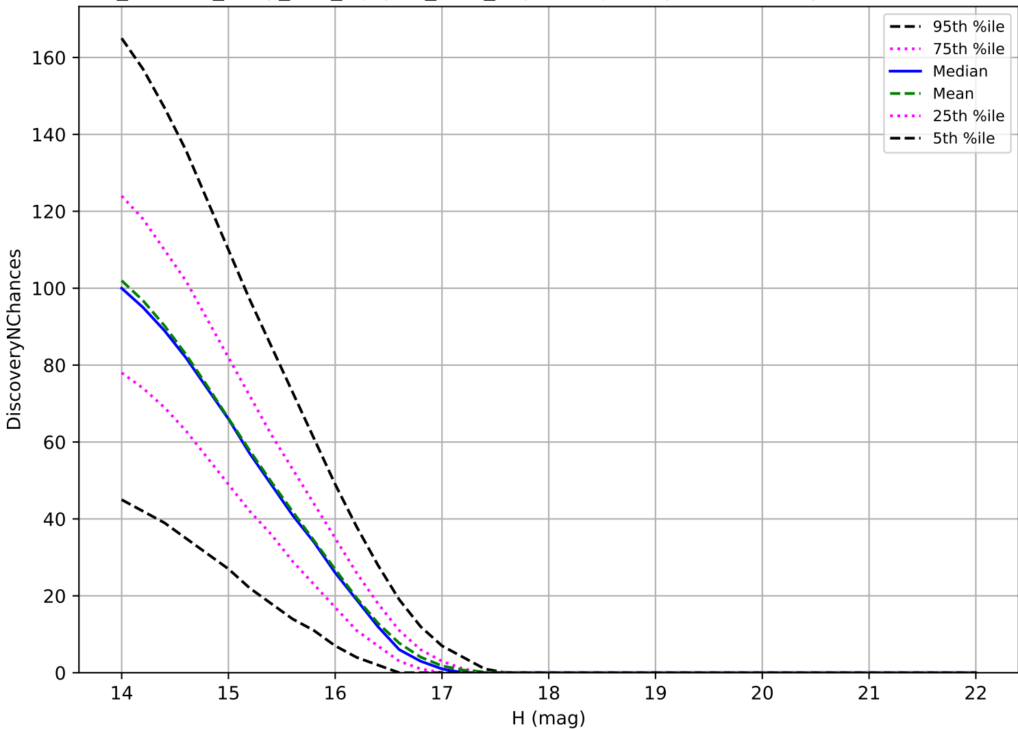
roll_uniform_early_half_mjdp67_v3.4_10yrs: Trojan 3 pairs in 15 nights detection loss
