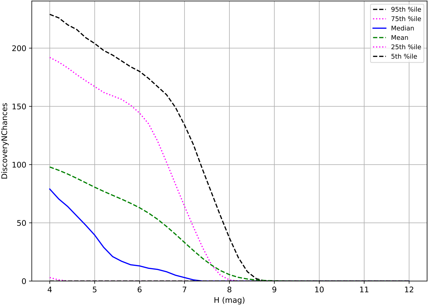
roll_uniform_early_half_mjdp67_v3.4_10yrs: TNO 3 pairs in 15 nights detection loss
