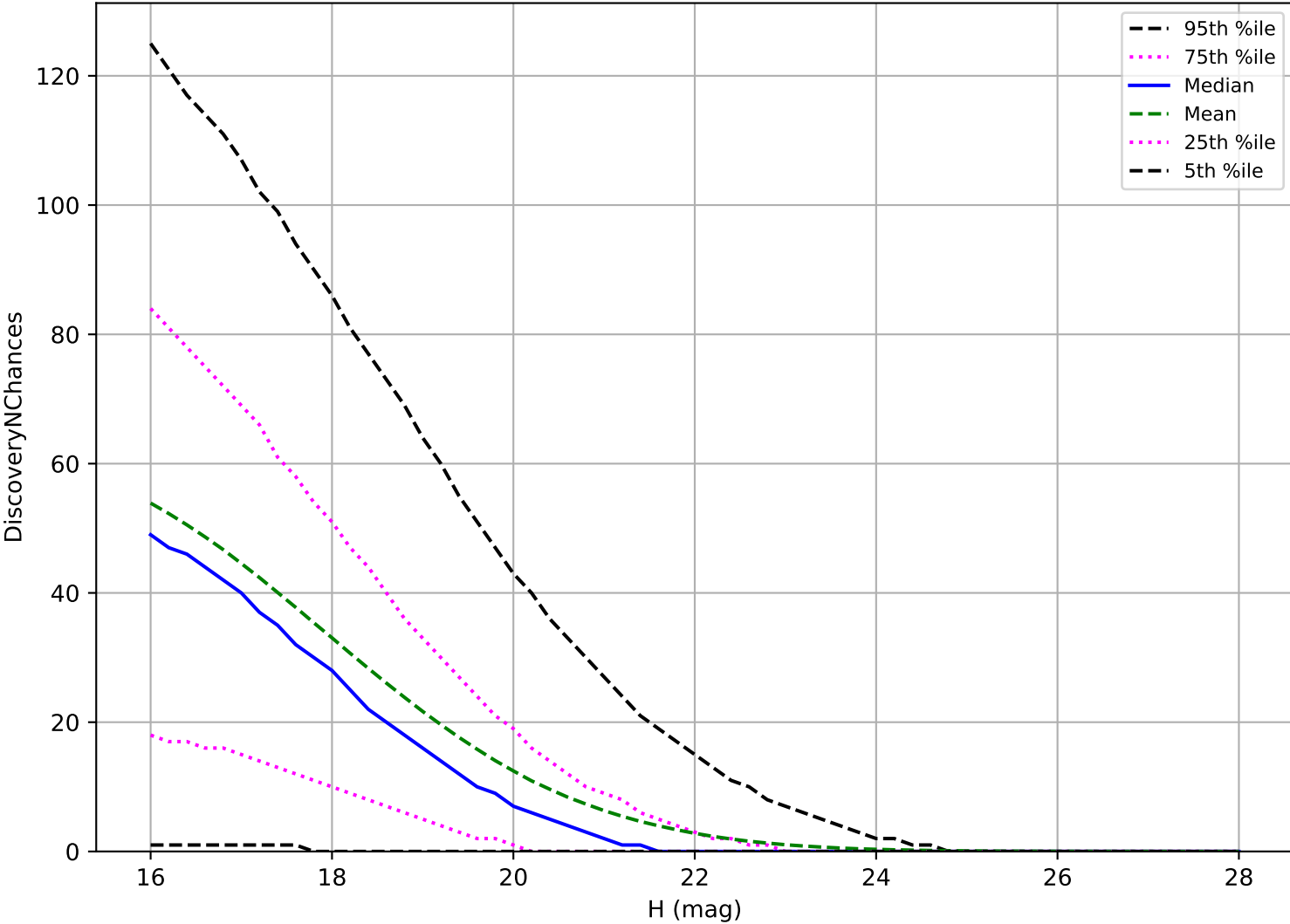
roll_uniform_early_half_mjdp67_v3.4_10yrs: PHA 3 pairs in 15 nights detection loss
