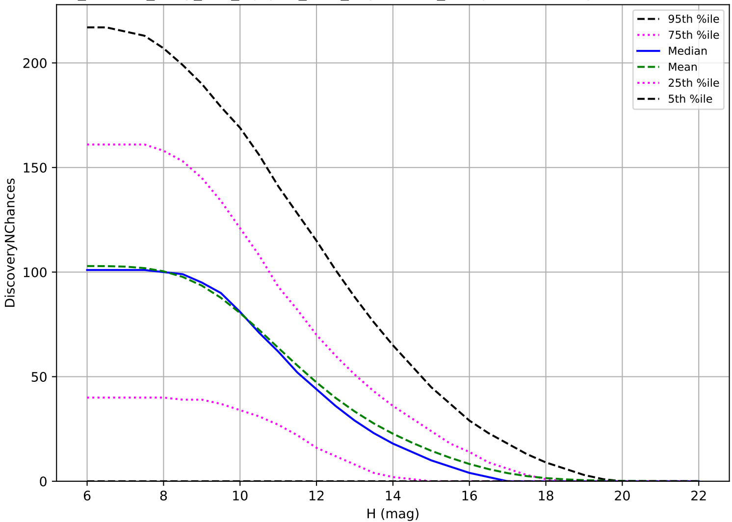
roll_uniform_early_half_mjdp67_v3.4_10yrs: OCC_r5 3 pairs in 15 nights detection loss
