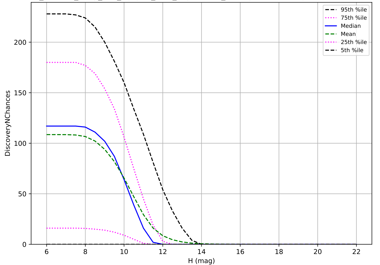
roll_uniform_early_half_mjdp67_v3.4_10yrs: OCC_r20 3 pairs in 15 nights detection loss
