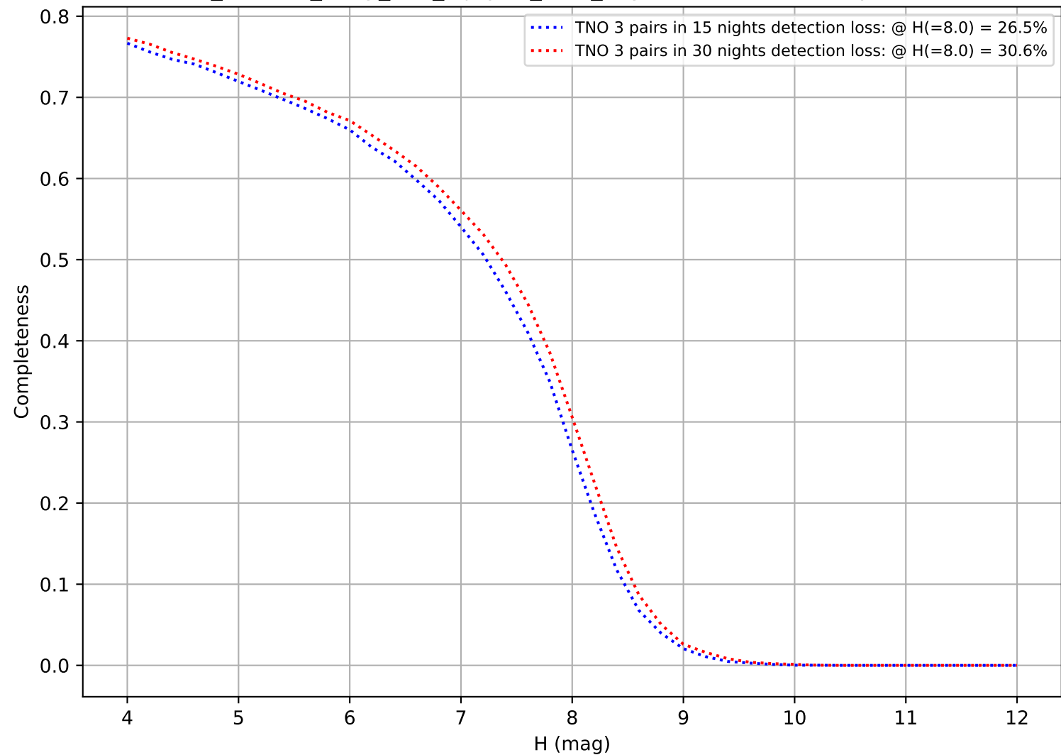
roll_uniform_early_half_mjdp67_v3.4_10yrs: DifferentialCompleteness
