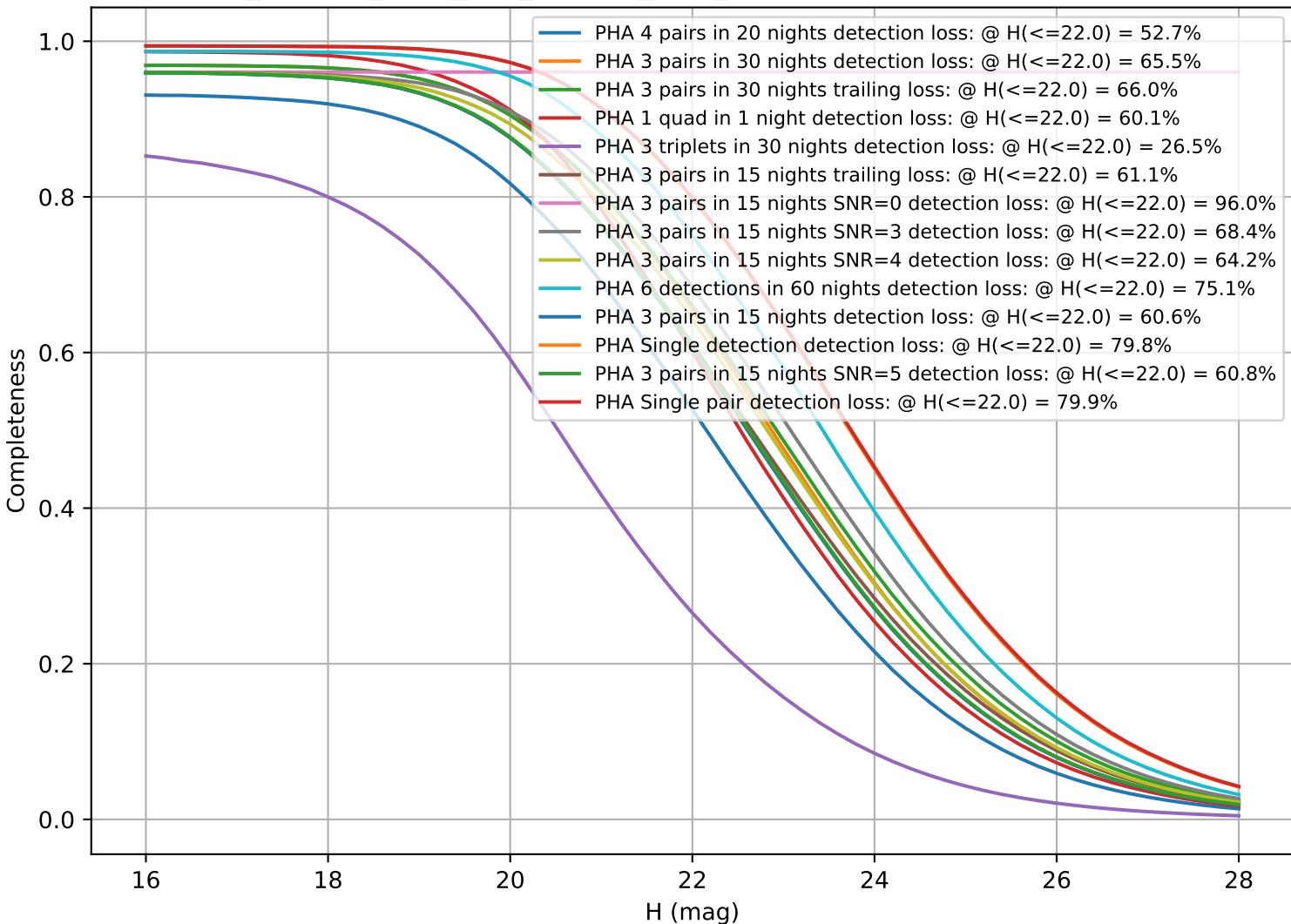
roll_uniform_early_half_mjdp67_v3.4_10yrs: CumulativeCompleteness
