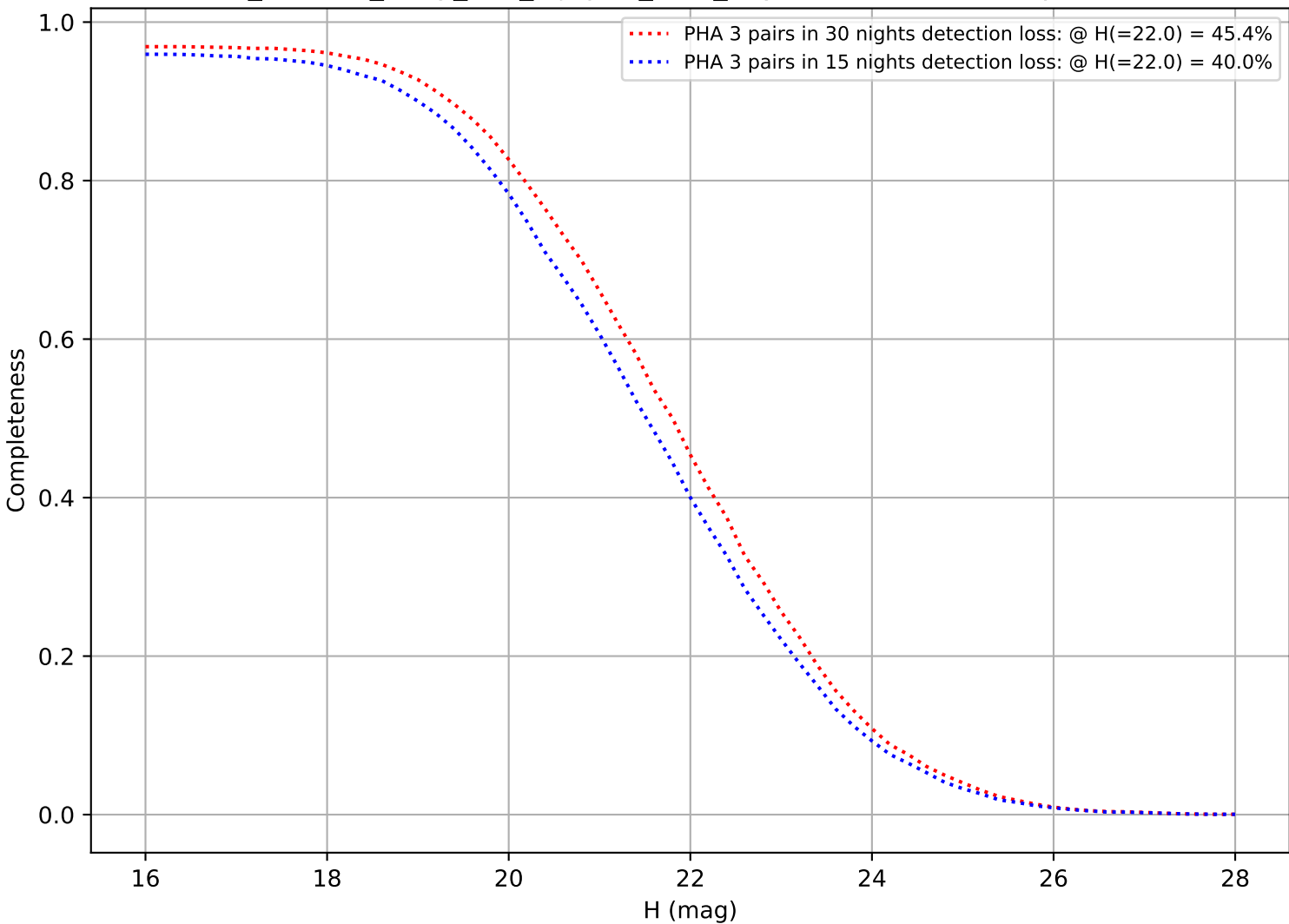
roll_uniform_early_half_mjdp67_v3.4_10yrs: DifferentialCompleteness
