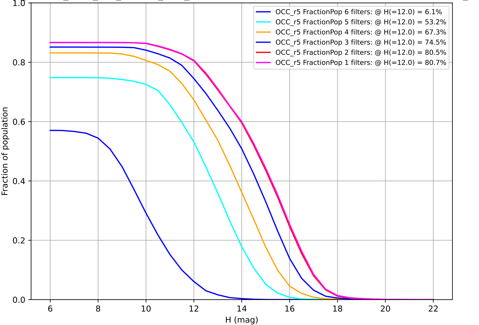
roll_uniform_early_half_mjdp67_v3.4_10yrs: Fraction of population with colors in X filters OCC_r5
