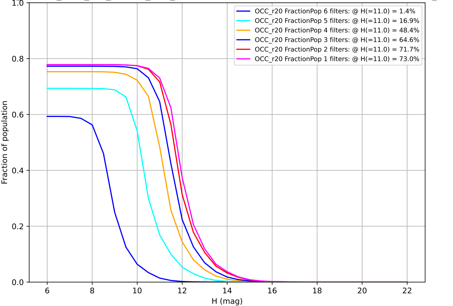
roll_uniform_early_half_mjdp67_v3.4_10yrs: Fraction of population with colors in X filters OCC_r20
