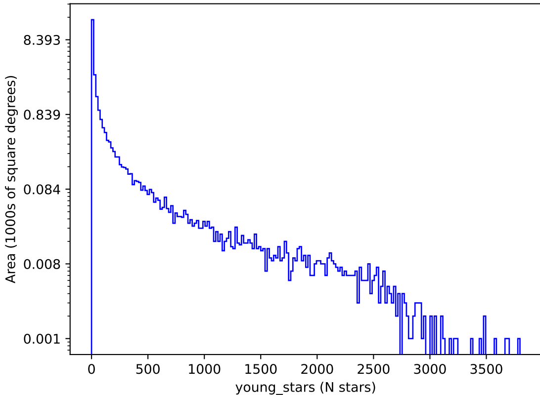
roll_uniform_early_half_mjdp67_v3.4_10yrs : young_stars
