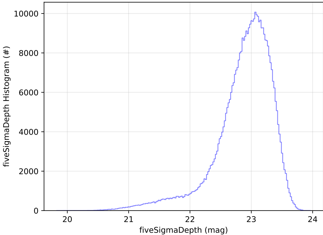
roll_uniform_early_half_mjdp67_v3.4_10yrs z: fiveSigmaDepth Histogram
