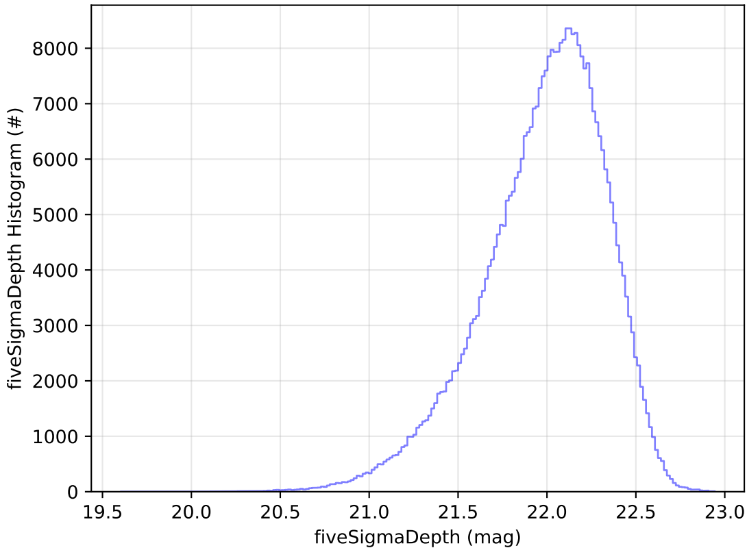
roll_uniform_early_half_mjdp67_v3.4_10yrs y: fiveSigmaDepth Histogram
